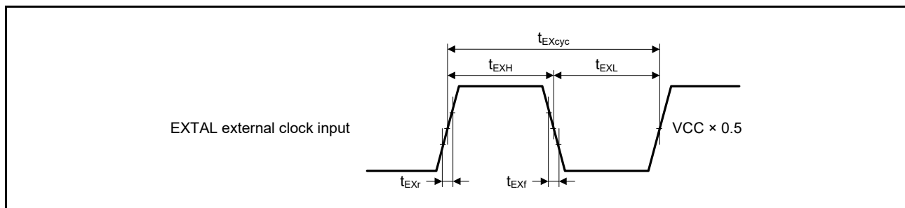
Figure 2.6 EXTERNAL external clock input timing
