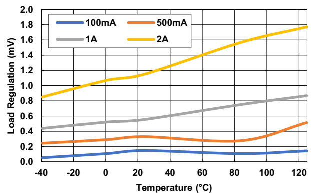
Figure 102. Load Regulation vs Temperature ( V_{IN} = 2.7V , V_{OUT} = 0.8V , \Delta I_{OUT} = 1mA to 2A )
