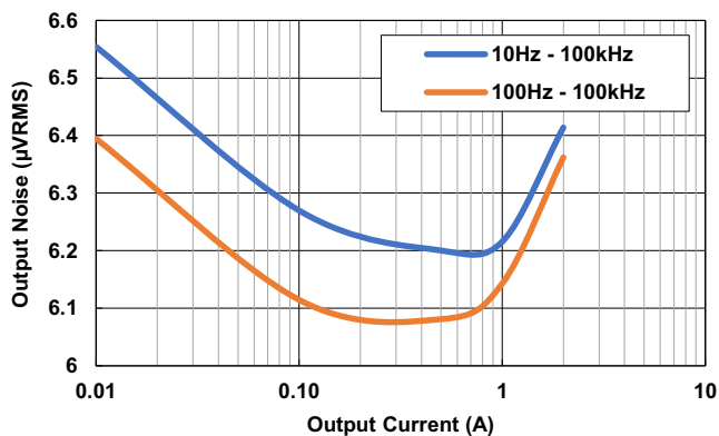
Figure 12. Integrated Output Noise vs I_{OUT} for Various Bandwidths ( V_{IN} = V_{OUT} + 1V , I_{OUT} = 2A )
