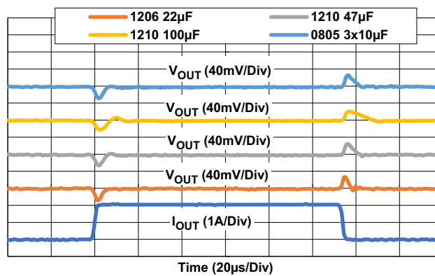
Figure 87. Load Transient Response for Various C_{OUT} ( V_{IN} = 3.9V , V_{OUT} = 3.3V , \Delta I_{OUT} = 100mA to 2A at 1A/\mu s )
