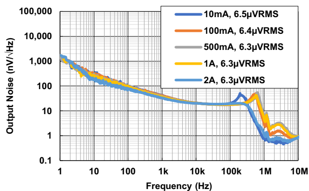
Figure 9. Output Noise vs Frequency for Various I_{OUT} ( V_{IN} = V_{OUT} + 500mV , I_{OUT} = 2A )
