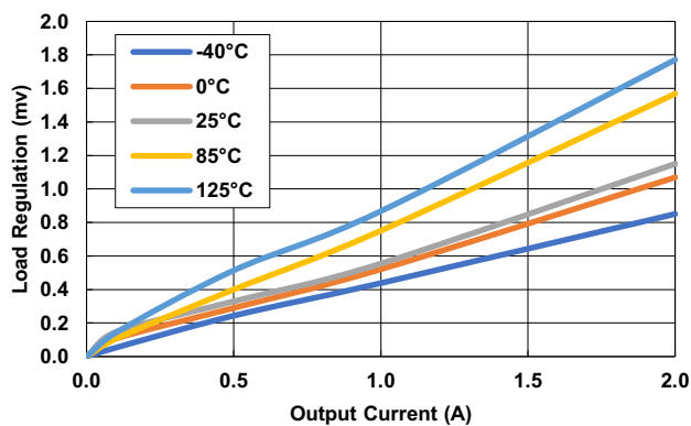
Figure 101. Load Regulation vs Output Current ( V_{IN} = 2.7V , V_{OUT} = 0.9V , \Delta I_{OUT} = 1mA to 2A )
