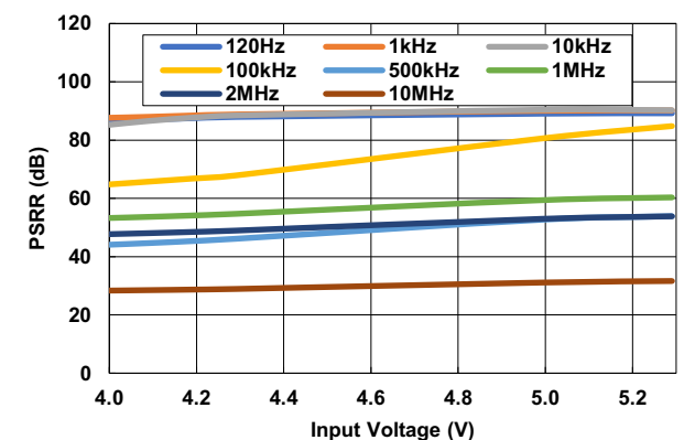
Figure 62. PSRR vs V_{IN} Various Frequencies ( V_{OUT} = 3.3V , I_{OUT} = 250mA )
