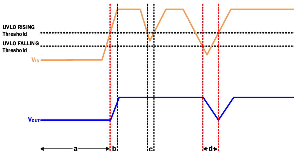
Figure 137. UVLO Operation
