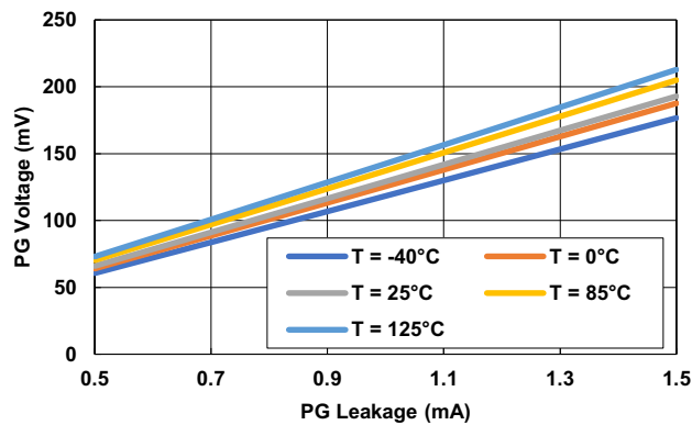
Figure 121. PG Voltage vs PG Sinking Current
