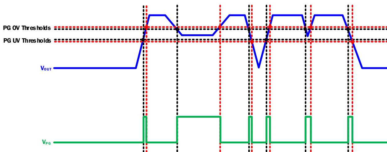
Figure 138. PG Operation
