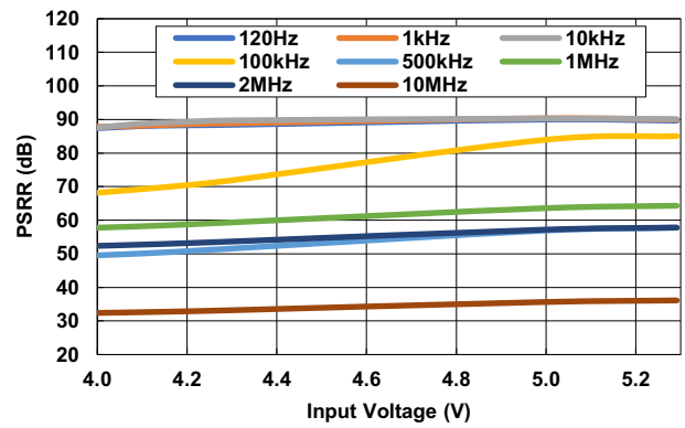
Figure 60. PSRR vs V_{IN} Various Frequencies ( V_{OUT} = 3.3V , I_{OUT} = 100mA )
