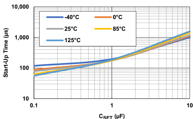
Figure 129. Start-Up Time vs C_{SET} for Various Temperatures ( V_{IN} = 5.5V , V_{OUT} = 1.8V , C_{SET} = 1\mu F , C_{OUT} = 22\mu F )
