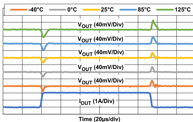
Figure 86. Load Transient Response for Various Temperatures ( V_{IN} = 3.9V , V_{OUT} = 3.3V , \Delta I_{OUT} = 100mA to 2A at 1A/\mu s )
