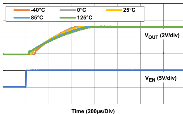
Figure 135. Start-Up Time for Various Temperatures ( V_{IN} = 5V , V_{OUT} = 3.3V , I_{OUT} = 2A , C_{SET} = 1\mu F , C_{OUT} = 22\mu F )
