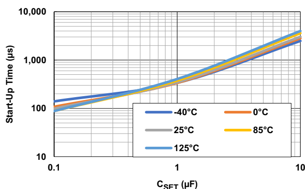
Figure 131. Start-Up Time vs C_{SET} for Various Temperatures ( V_{IN} = 5.5V , V_{OUT} = 3.3V , C_{SET} = 1\mu F , C_{OUT} = 22\mu F )
