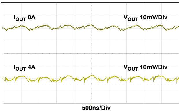
Figure 11. Output Ripple, V_{IN} = 5\text{V} , V_{OUT} = 1.8\text{V} , f_{SW} = 1.5\text{MHz} , C_{OUT} = 2 \times 22\mu\text{F} Ceramic
