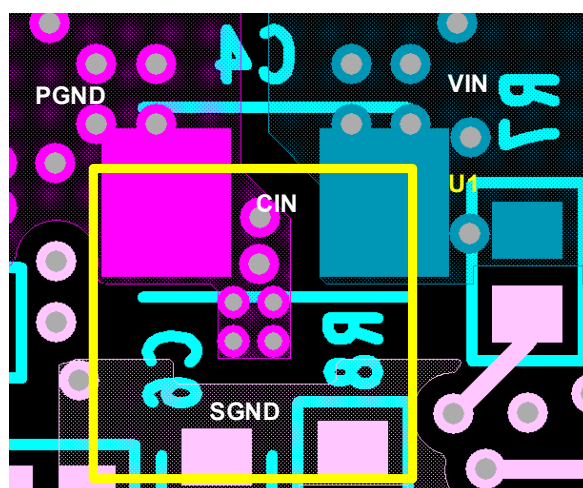
Figure 37. Layout Example - Bottom Layer
