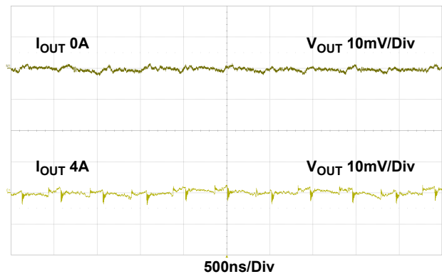
Figure 13. Output Ripple, V_{IN} = 3.3\text{V} , V_{OUT} = 0.8\text{V} , f_{SW} = 2\text{MHz} , C_{OUT} = 2 \times 22\mu\text{F} Ceramic
