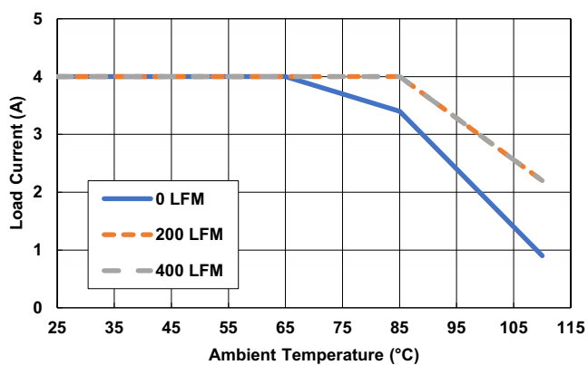
Figure 32. V_{IN} = 5\text{V} , V_{OUT} = 2.5\text{V} , f_{SW} = 1.8\text{MHz}
