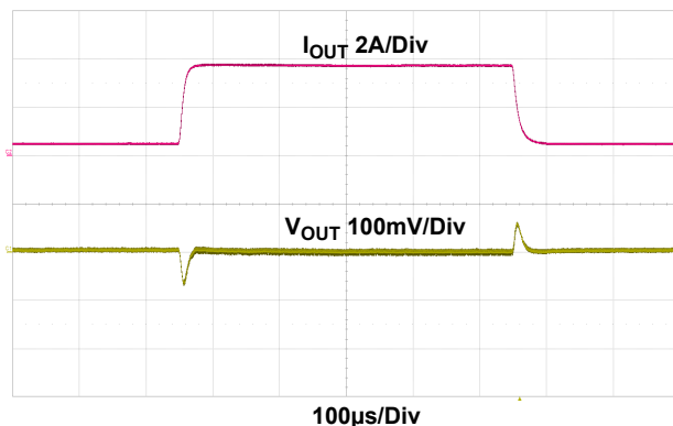
Figure 18. V_{IN} = 5\text{V} , V_{OUT} = 1.2\text{V} , f_{SW} = 1.2\text{MHz} , C_{OUT} = 2 \times 22\mu\text{F} Ceramic
