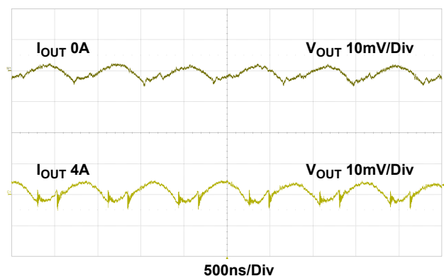
Figure 10. Output Ripple, V_{IN} = 5\text{V} , V_{OUT} = 1.2\text{V} , f_{SW} = 1.2\text{MHz} , C_{OUT} = 2 \times 22\mu\text{F} Ceramic
