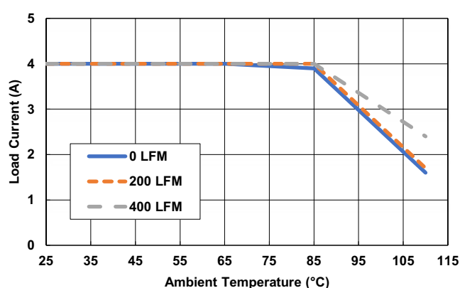
Figure 30. V_{IN} = 5\text{V} , V_{OUT} = 1.2\text{V} , f_{SW} = 1.2\text{MHz}
