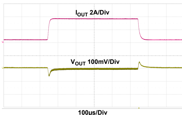
Figure 20. V_{IN} = 5\text{V} , V_{OUT} = 3.3\text{V} , f_{SW} = 2.4\text{MHz} , C_{OUT} = 2 \times 22\mu\text{F} Ceramic
