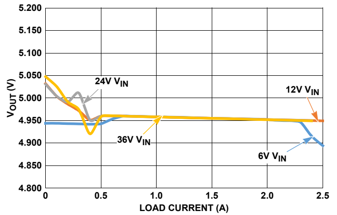
FIGURE 10. LOAD REGULATION, V_{OUT} = 5V , T_A = +25^\circ C
