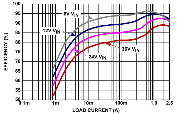
FIGURE 8. EFFICIENCY, SYNCHRONOUS BUCK, PFM MODE, V_{OUT} = 5V , T_A = +25^\circ C
