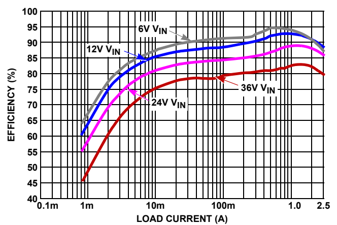
FIGURE 12. EFFICIENCY, SYNCHRONOUS BUCK, PFM MODE, V_{OUT} = 3.3V , T_A = +25^\circ C
