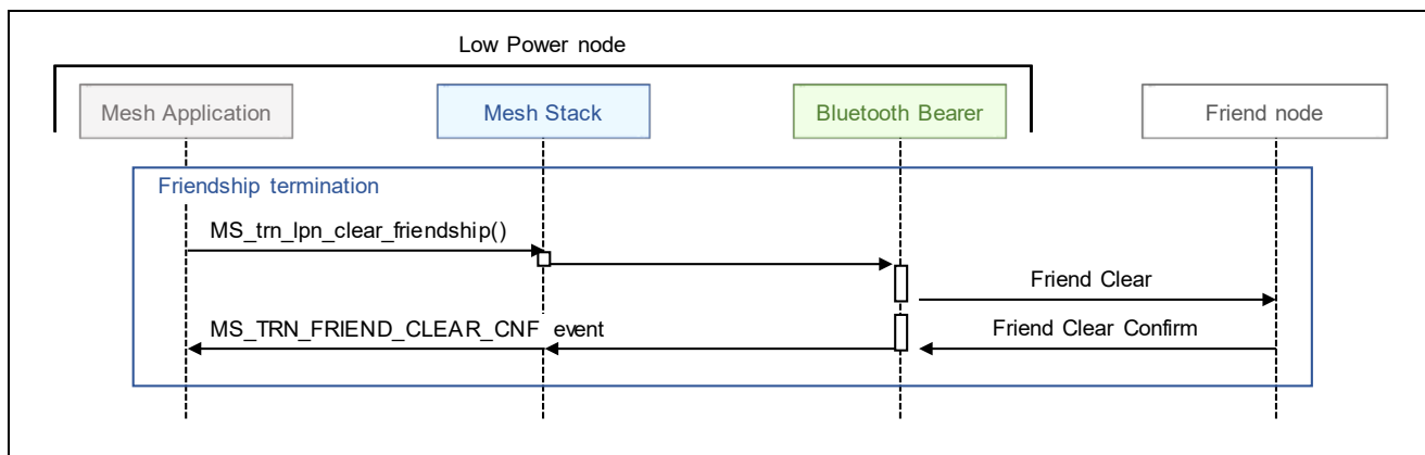
Figure 3-11 Friendship Termination
