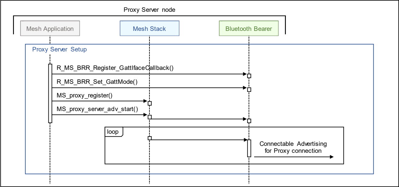
Figure 3-7 Proxy Setup
