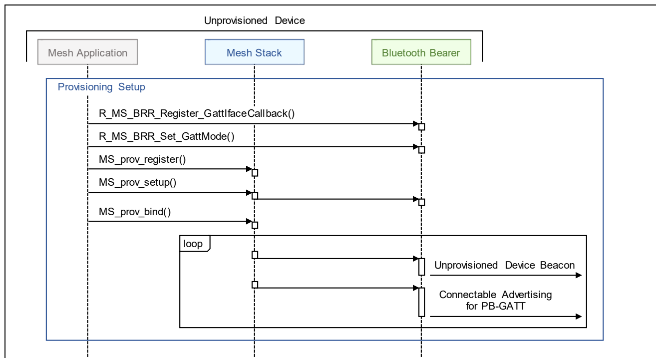
Figure 3-2 Provisioning Setup
