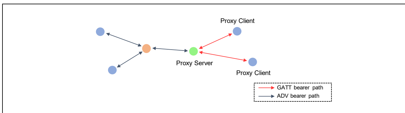
Figure 1-9 Proxy
