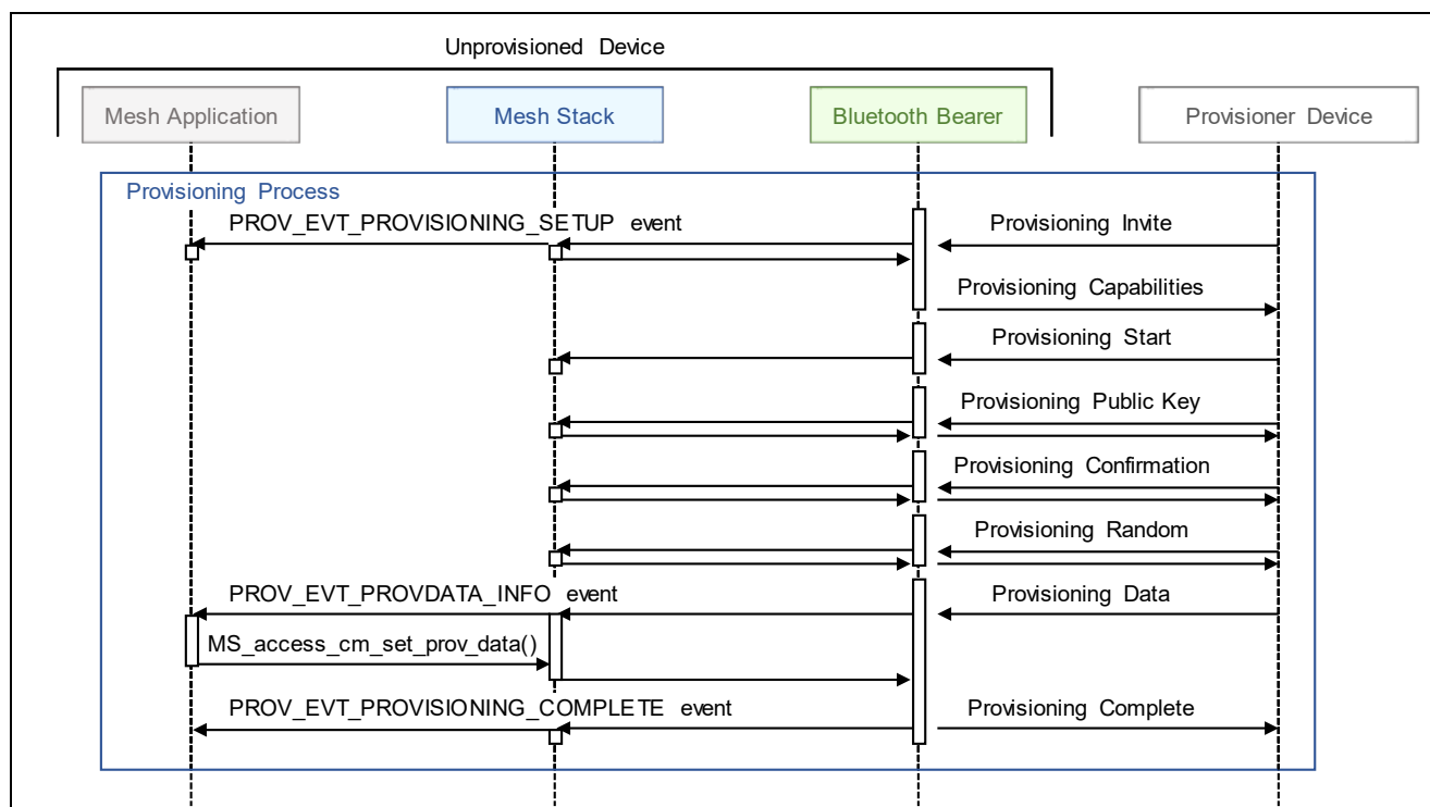
Figure 3-5 Provisioning Process
