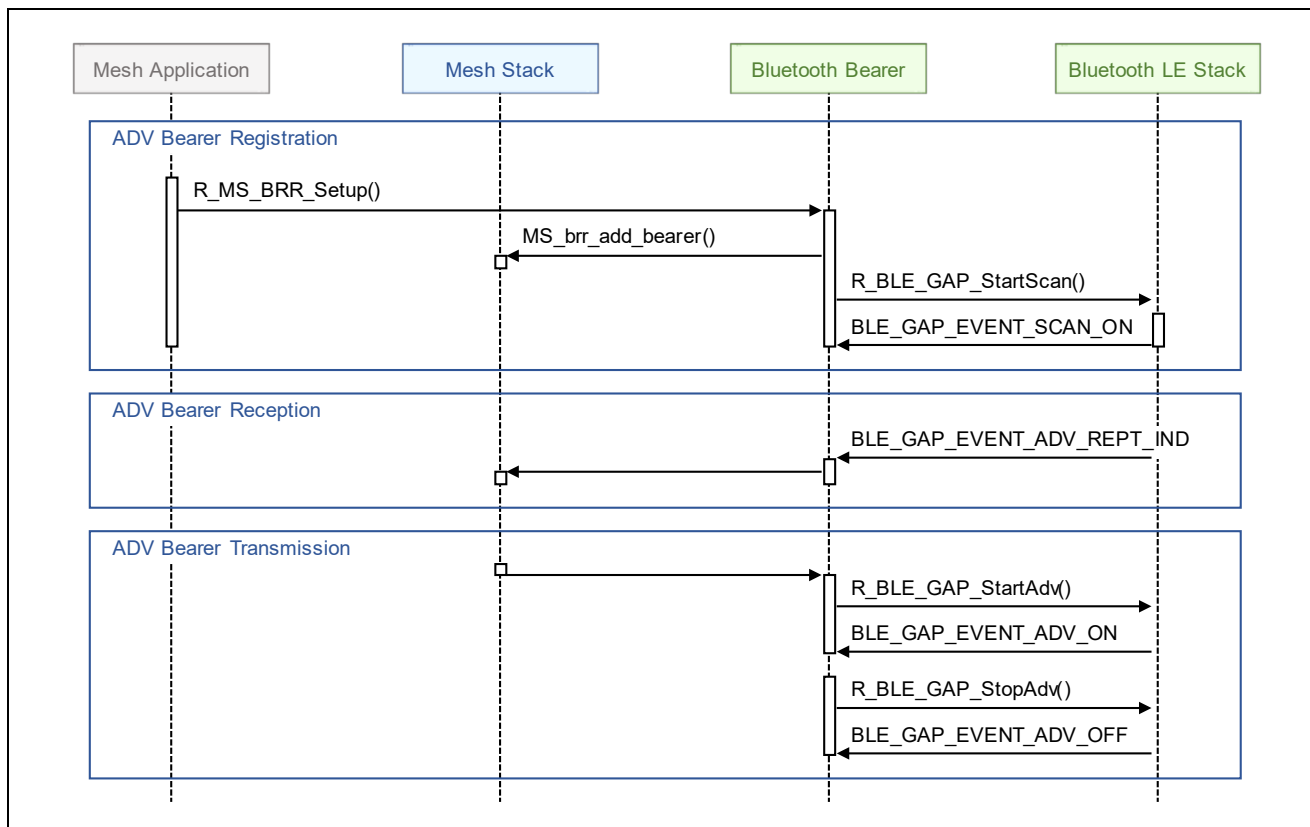
Figure 2-5 ADV Bearer Operation
