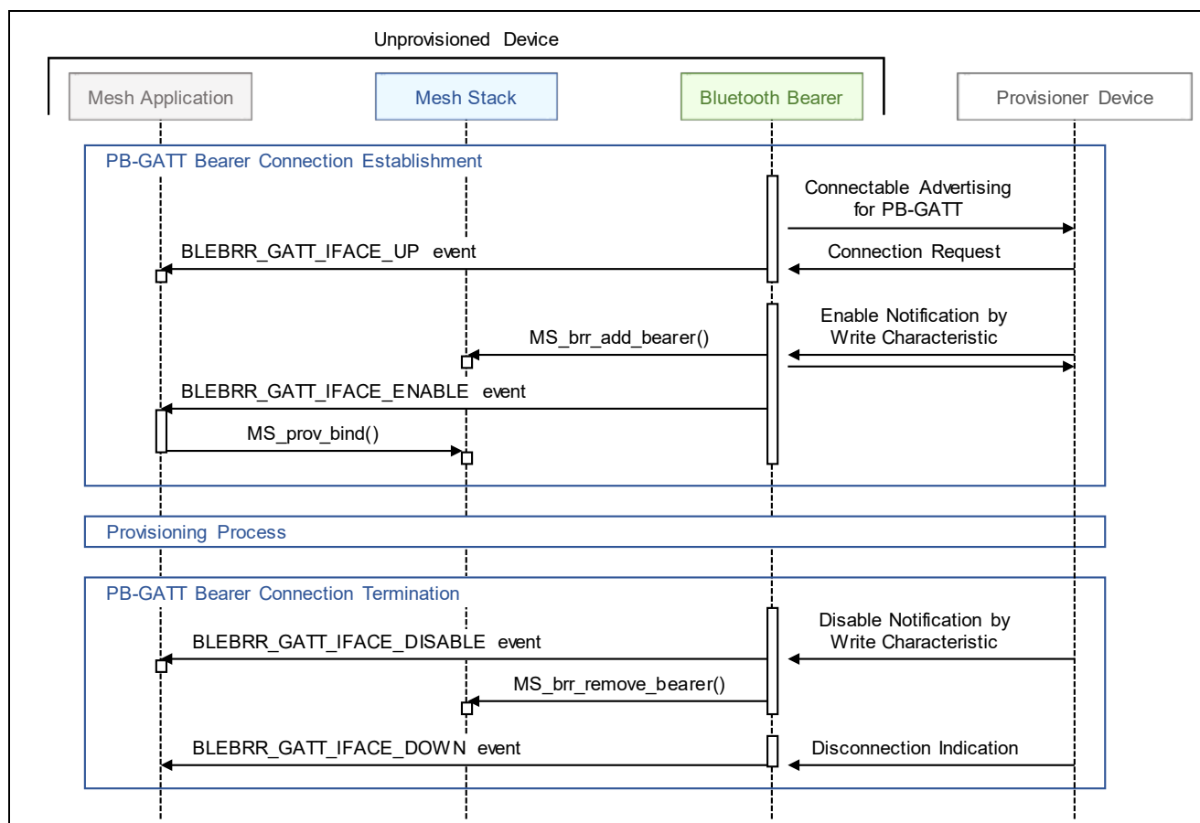
Figure 3-4 Connection Establishment over PB-GATT
