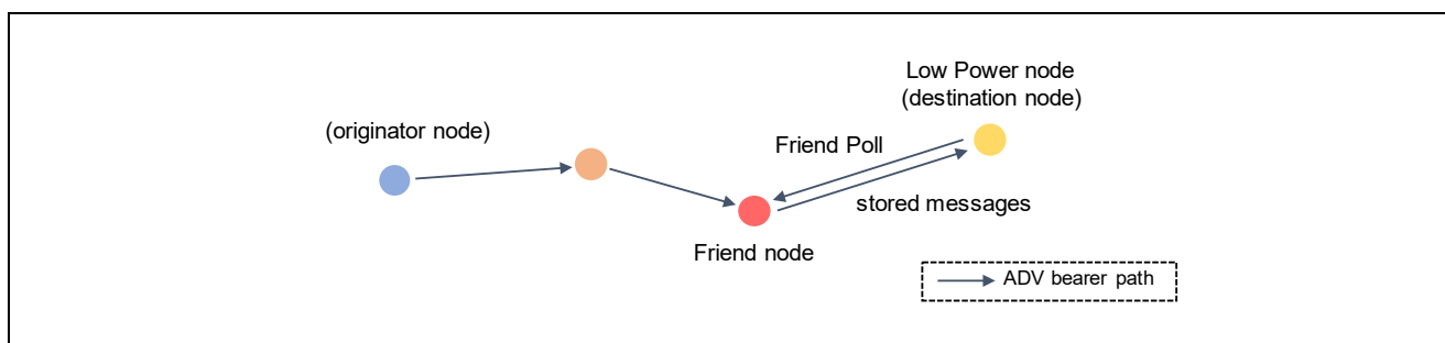
Figure 1-10 Friendship
