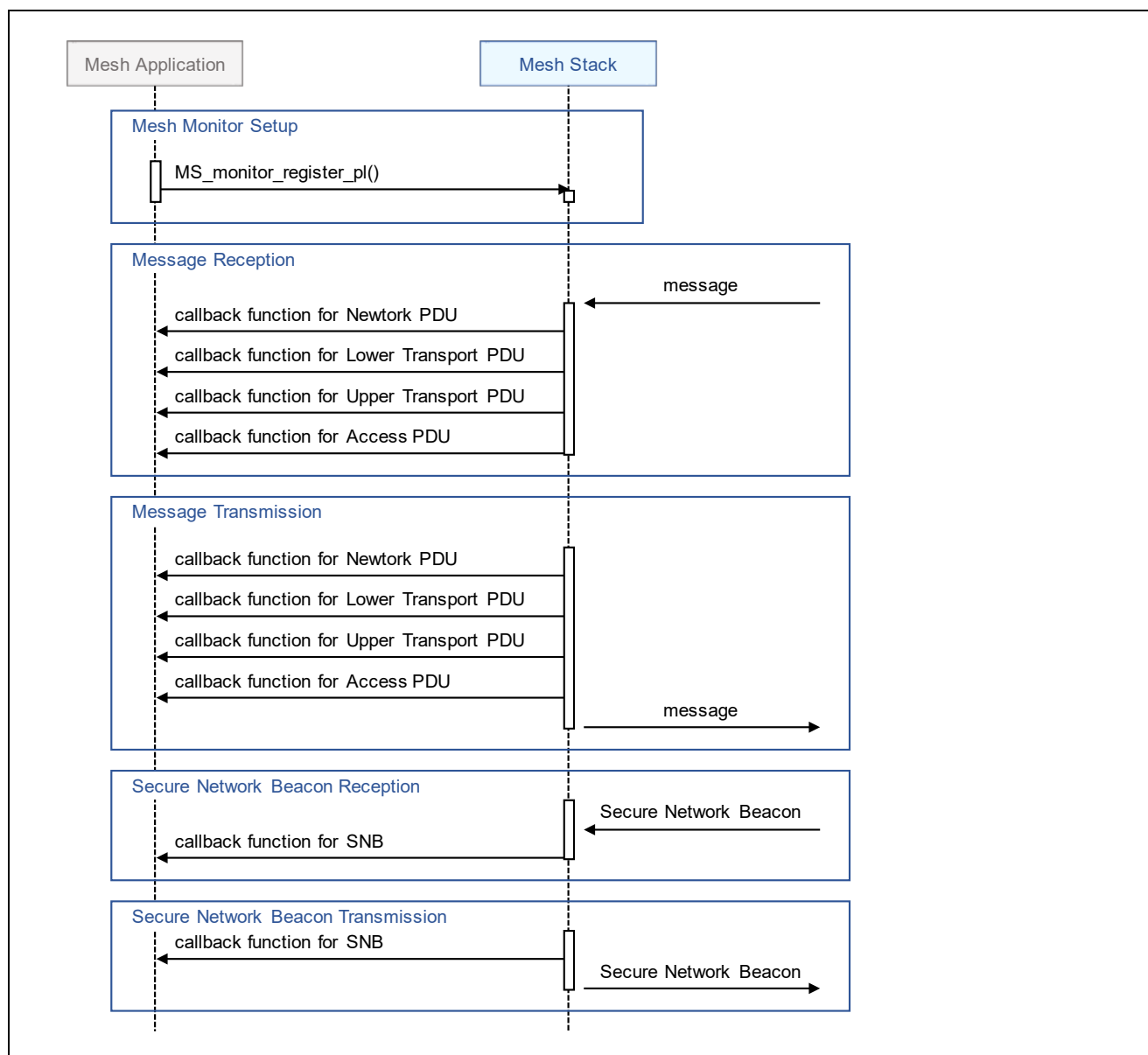
Figure 3-18 Mesh Monitoring
